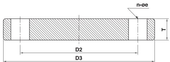
DN15~DN600 BLIND FLANGE
