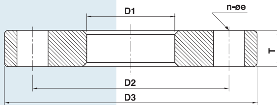
DN15~DN600 WELDING FLANGE
