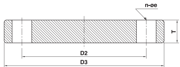
DN15~DN600 BLIND FLANGE
